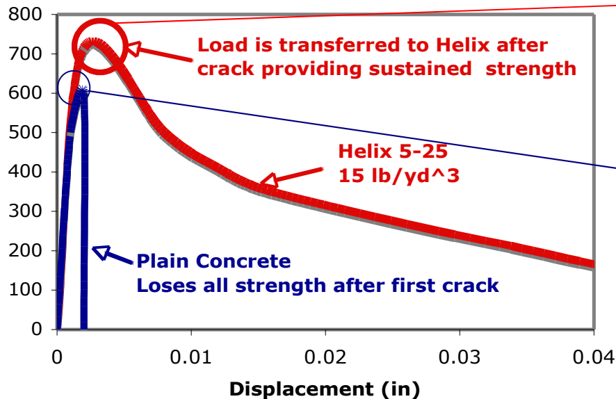
Helix Reinforced Versus Plain Concrete
